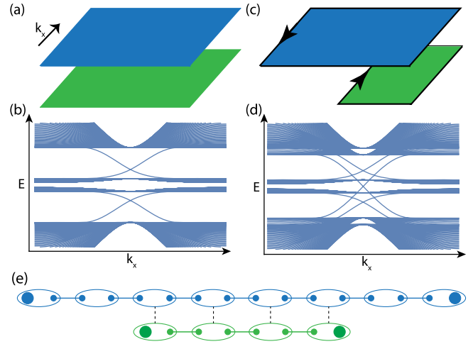
FIG. 2. Topological proximity effect of a Chern insulator. (a) A bilayer slab (in-)finite in the (x) y direction, with the spectrum shown in (b). (c) A “terrace” in which the left boundary of A is separated from that of B . (d) The resulting spectrum, with weakly coupled counterpropagating edge states in the bulk gap localized at the distinct boundaries. (e) Schematic of a Kitaev wire BTPE. Note the original Majorana zero modes (the large blue dots) and the new Majorana modes (the large green dots).
